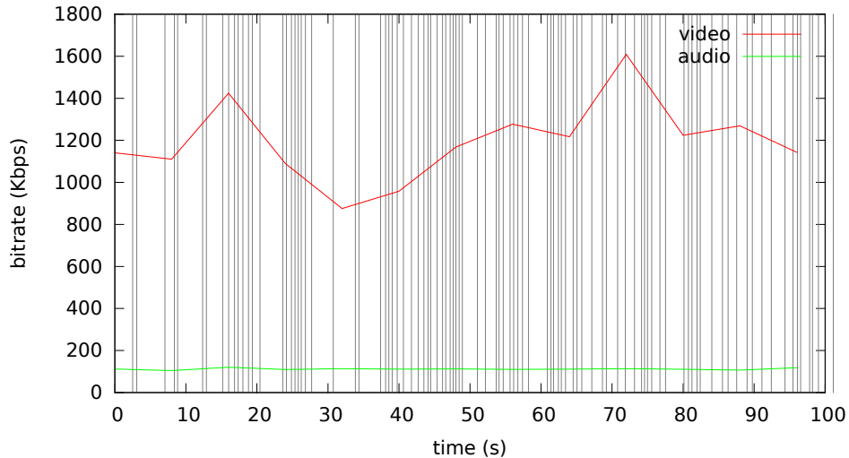
Bitrate analysis of videos-default/movietrailer-default.mp4
