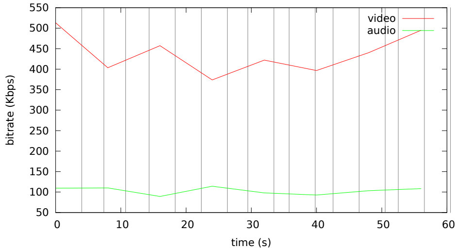
Bitrate analysis of videos-default/crap-default.mp4
