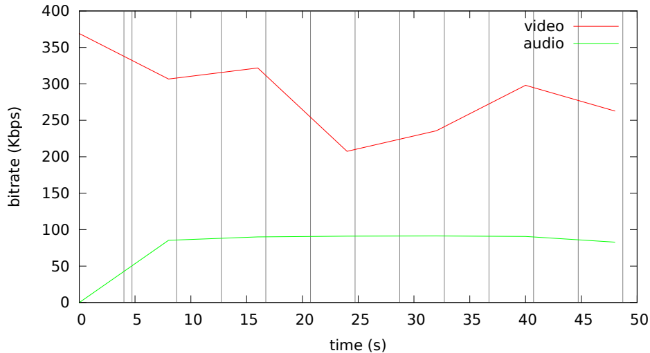
Bitrate analysis of videos-default/interview-default.mp4
