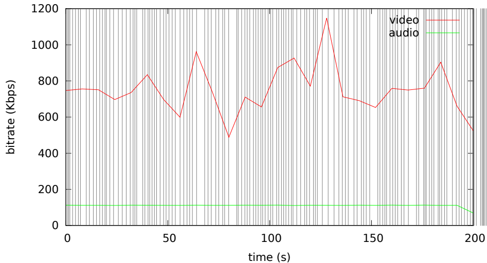
Bitrate analysis of videos-default/blackwhite-default.mp4
