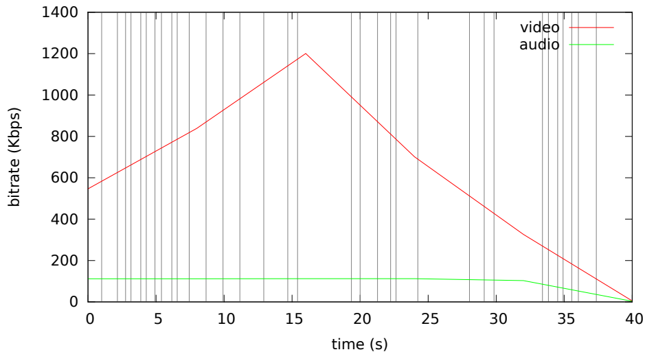
Bitrate analysis of videos-default/motiongraphics-default.mp4
