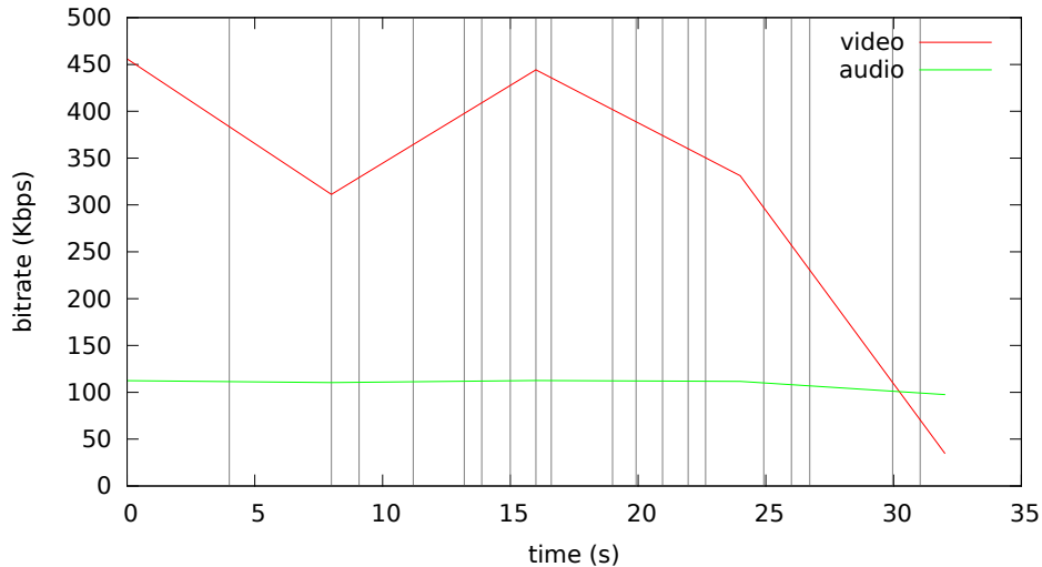
Bitrate analysis of videos-default/animation-default.mp4
