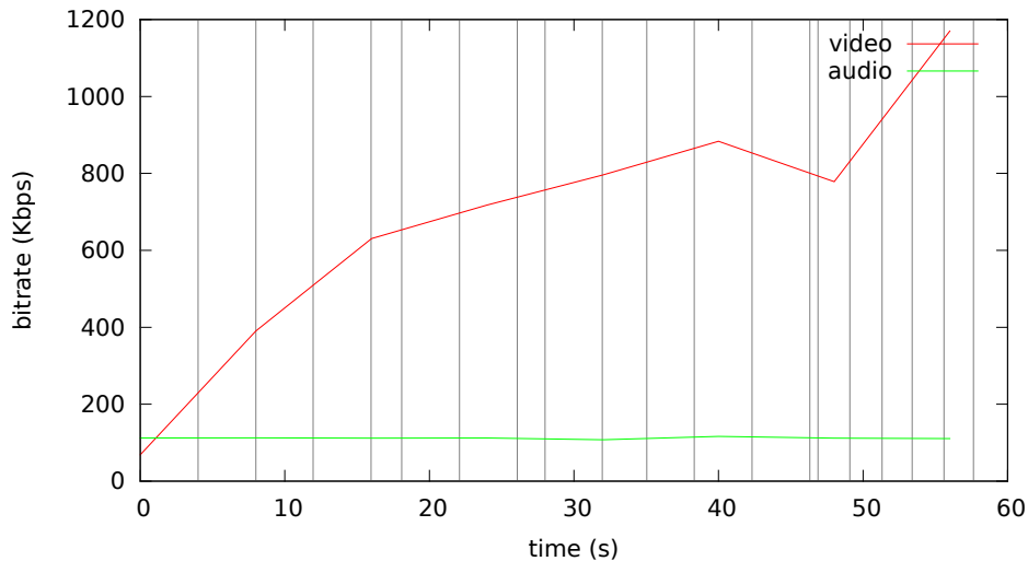
Bitrate analysis of videos-default/presentation-default.mp4
