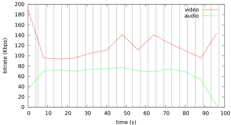
Bitrate analysis of videos-default/screencast-default.mp4
