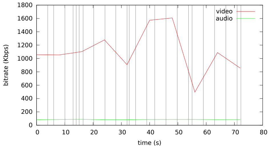
Bitrate analysis of videos-default/soccer-default.mp4
