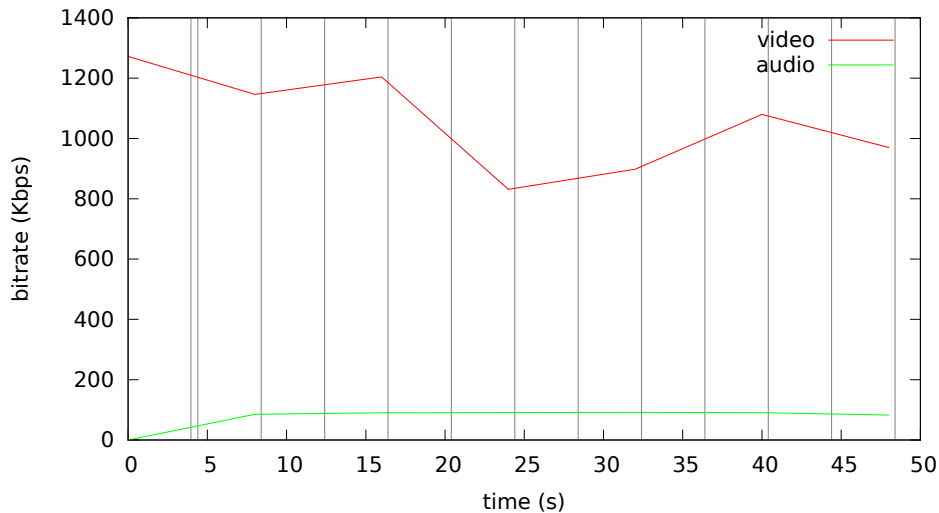
Bitrate analysis of videos-default2/interview-default2.mp4
