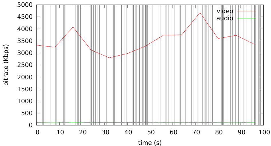
Bitrate analysis of videos-default2/movietrailer-default2.mp4
