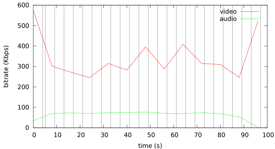
Bitrate analysis of videos-default2/screencast-default2.mp4
