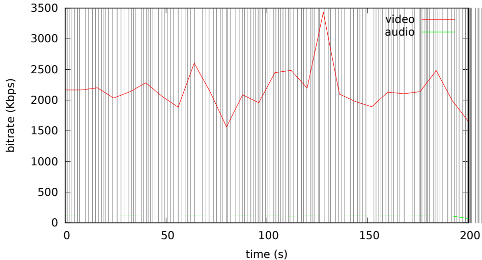
Bitrate analysis of videos-default2/blackwhite-default2.mp4
