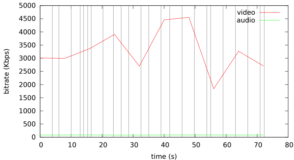
Bitrate analysis of videos-default2/soccer-default2.mp4
