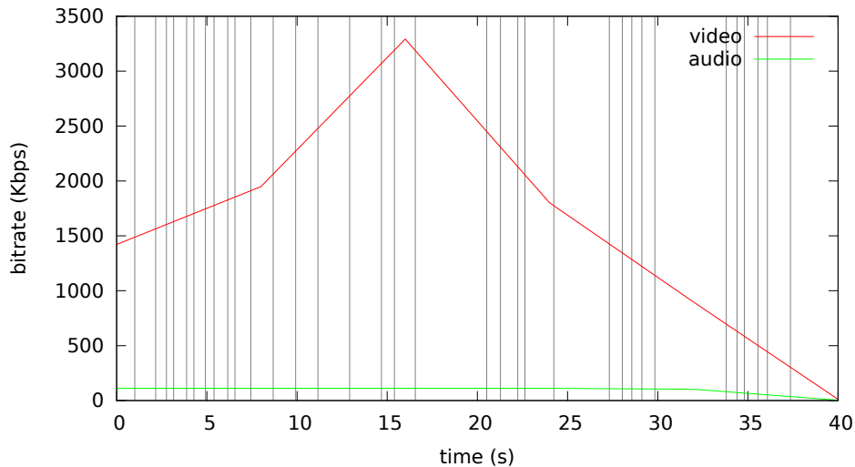
Bitrate analysis of videos-default2/motiongraphics-default2.mp4
