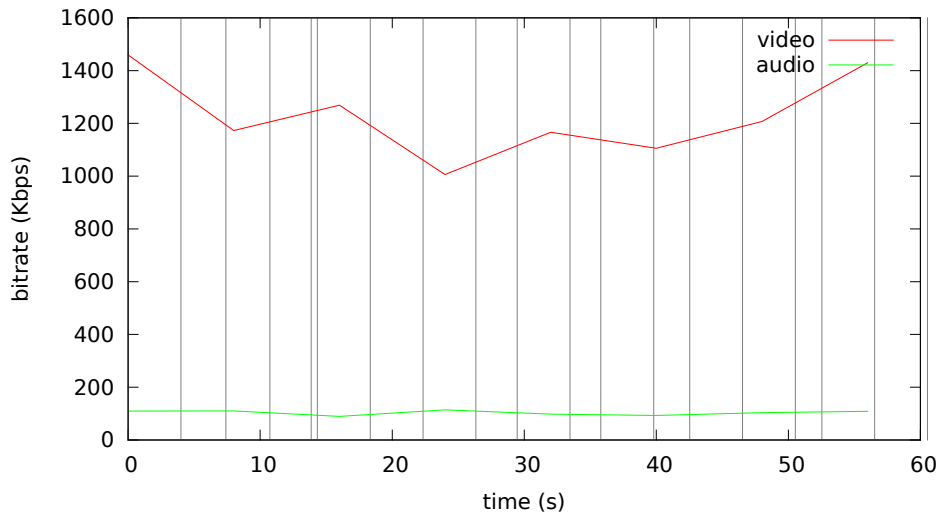
Bitrate analysis of videos-default2/crap-default2.mp4
