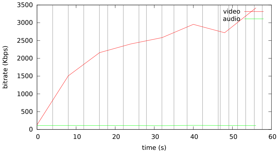
Bitrate analysis of videos-default2/presentation-default2.mp4
