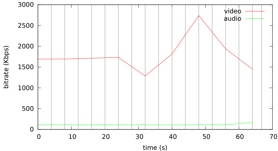
Bitrate analysis of videos-default2/fluidmotion-default2.mp4
