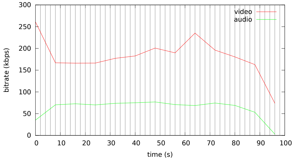
Bitrate analysis of videos-keyint2s/screencast-keyint2s.mp4
