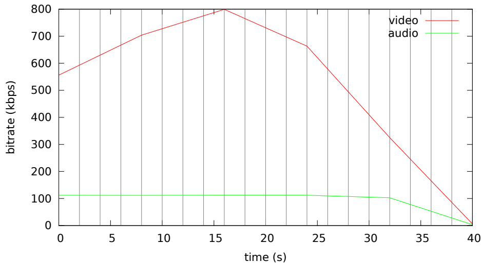
Bitrate analysis of videos-keyint2s/motiongraphics-keyint2s.mp4
