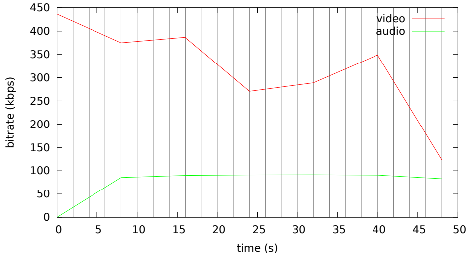
Bitrate analysis of videos-keyint2s/interview-keyint2s.mp4
