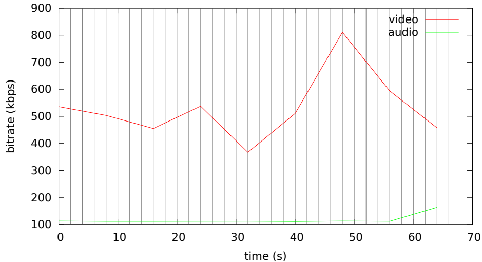
Bitrate analysis of videos-keyint2s/fluidmotion-keyint2s.mp4
