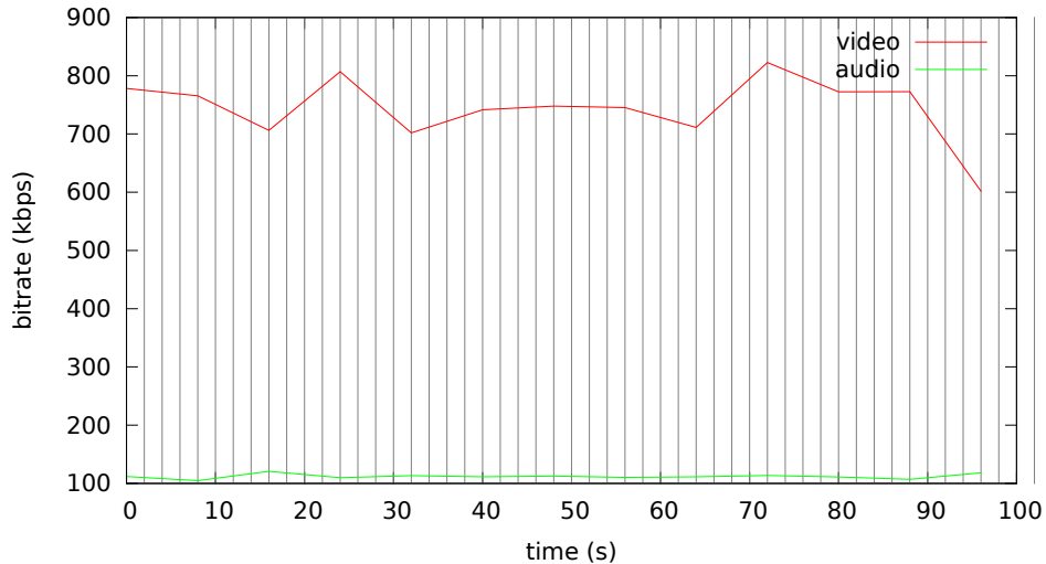
Bitrate analysis of videos-keyint2s/movietrailer-keyint2s.mp4
