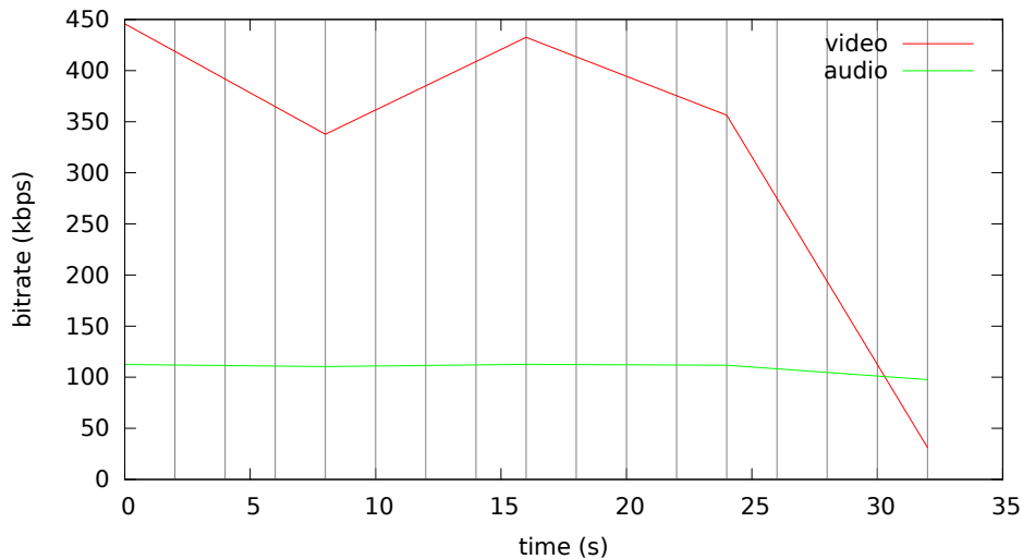
Bitrate analysis of videos-keyint2s/animation-keyint2s.mp4
