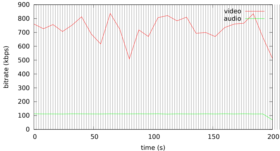
Bitrate analysis of videos-keyint2s/blackwhite-keyint2s.mp4
