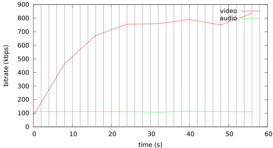
Bitrate analysis of videos-keyint2s/presentation-keyint2s.mp4
