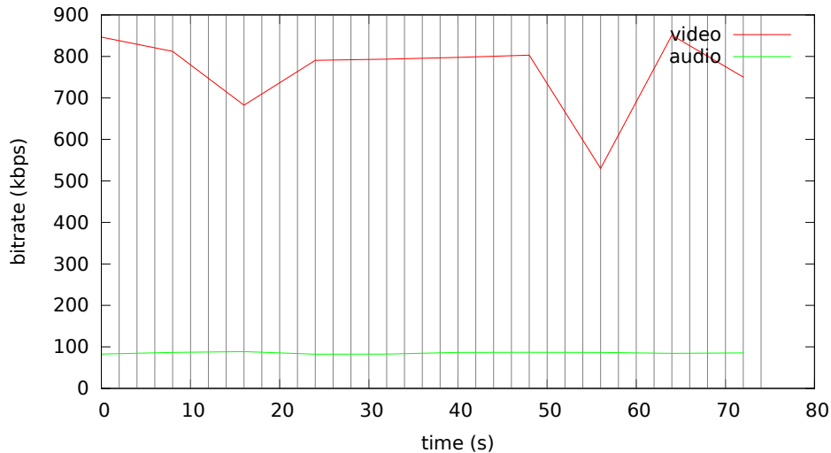
Bitrate analysis of videos-keyint2s/soccer-keyint2s.mp4
