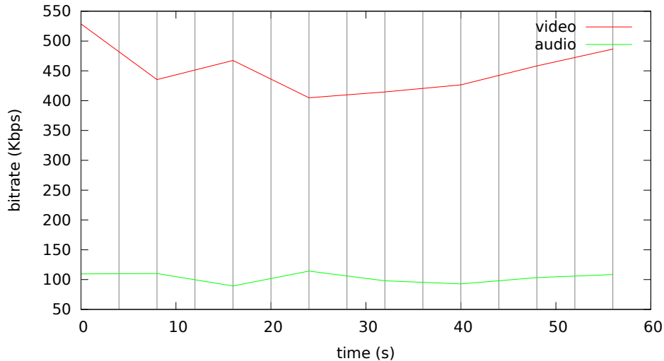
Bitrate analysis of videos-vbv/crap-vbv.mp4
