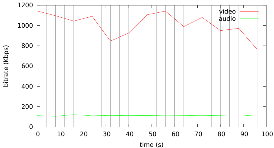
Bitrate analysis of videos-vbv/movietrailer-vbv.mp4
