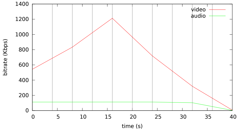
Bitrate analysis of videos-vbv/motiongraphics-vbv.mp4
