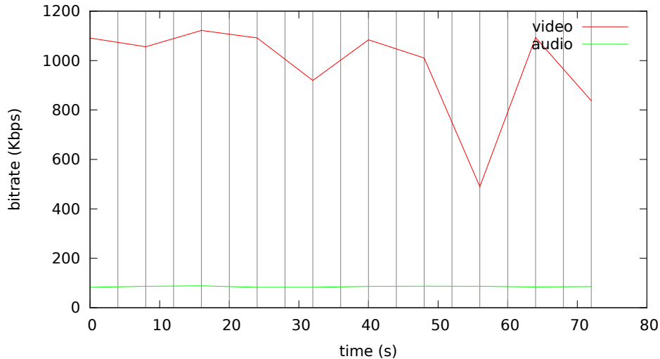
Bitrate analysis of videos-vbv/soccer-vbv.mp4
