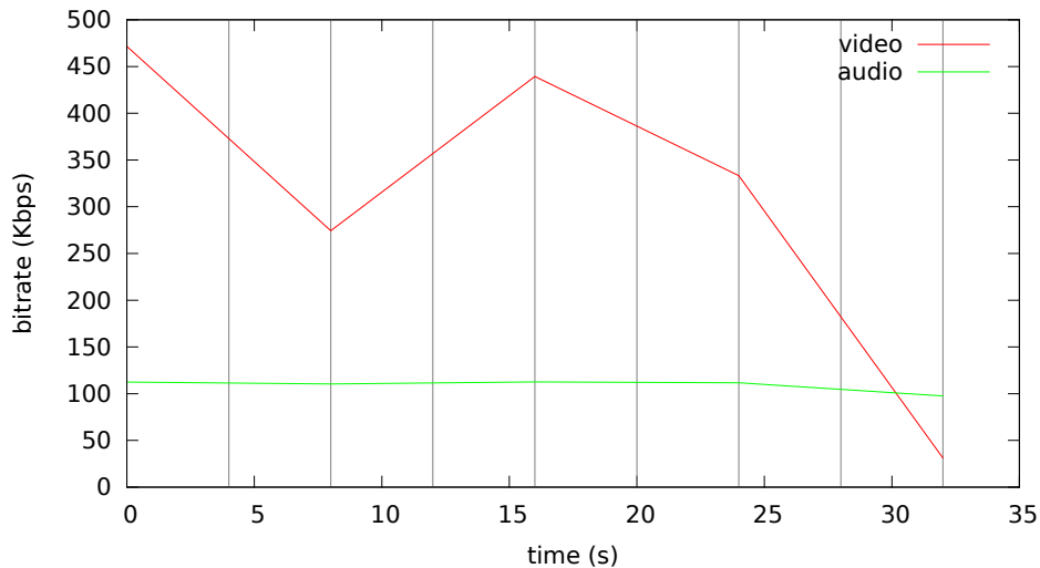
Bitrate analysis of videos-vbv/animation-vbv.mp4
