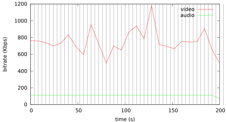
Bitrate analysis of videos-vbv/blackwhite-vbv.mp4
