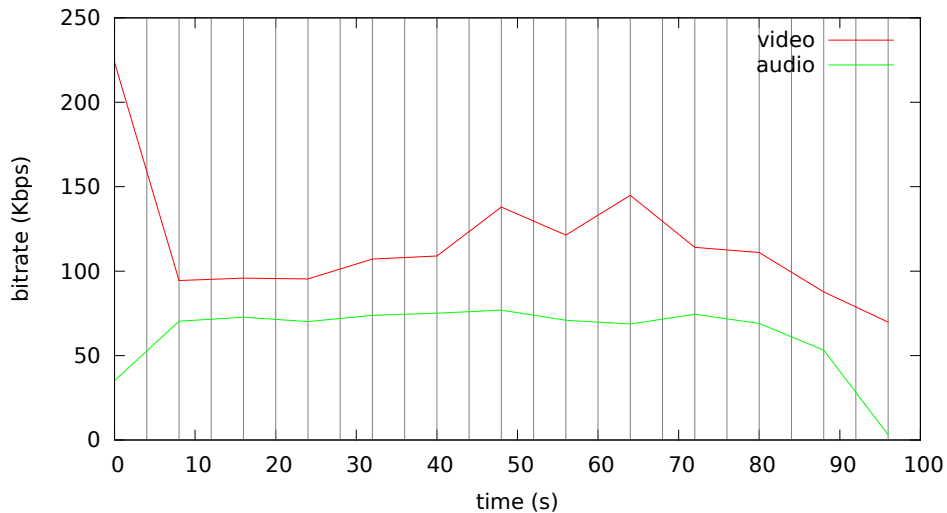
Bitrate analysis of videos-vbv/screencast-vbv.mp4
