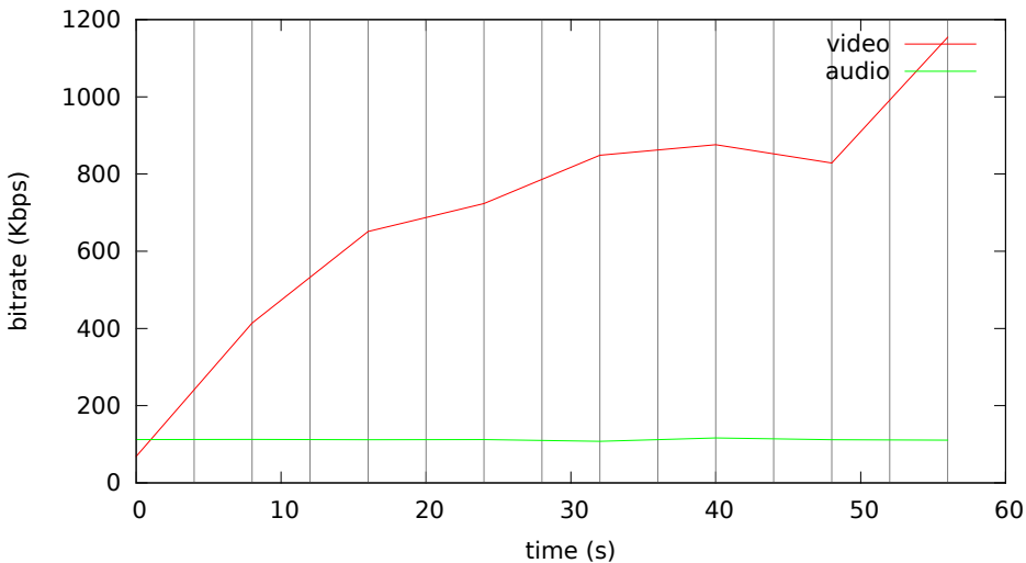
Bitrate analysis of videos-vbv/presentation-vbv.mp4
